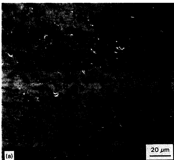
Figure 3 SEM photographs obtained after light etching of the \text{Ni}_3\text{Al} of this work.
