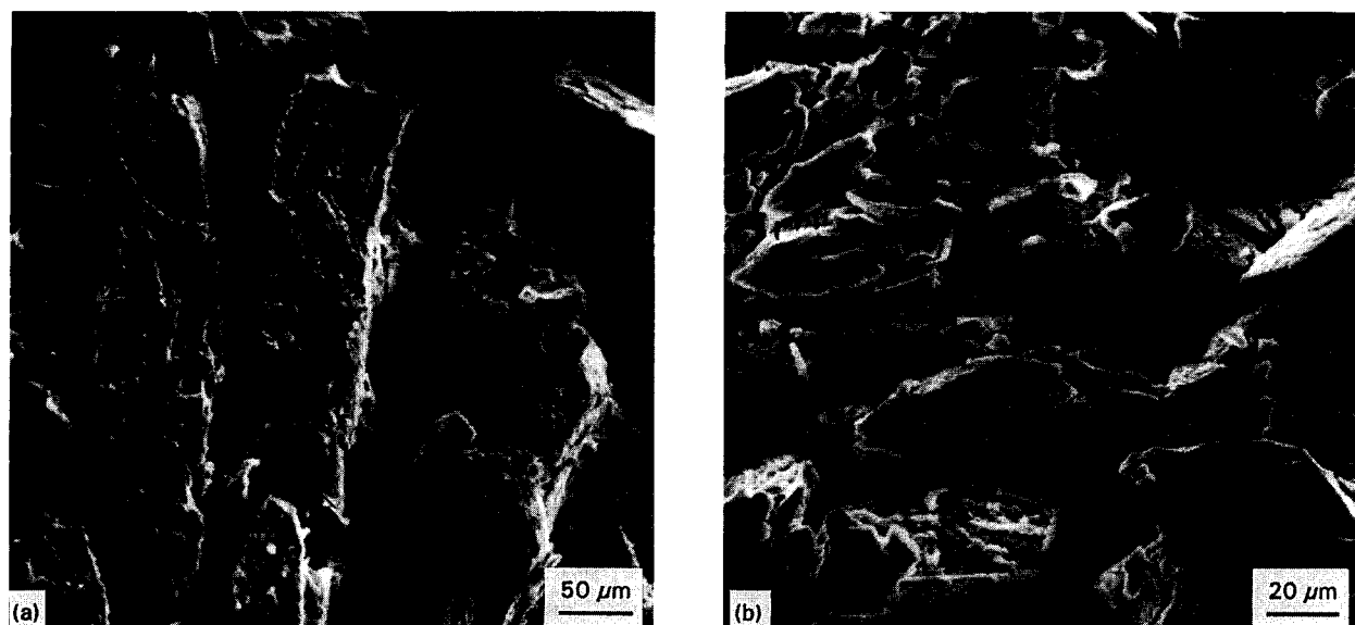
Figure 6 SEM photographs obtained after deep etching of (a) the needle-shaped \text{NiAl}_3 grains in the excess aluminium region, and (b) the equiaxed \text{NiAl}_3 grains in the \text{Al/NiAl}_3 composite.
