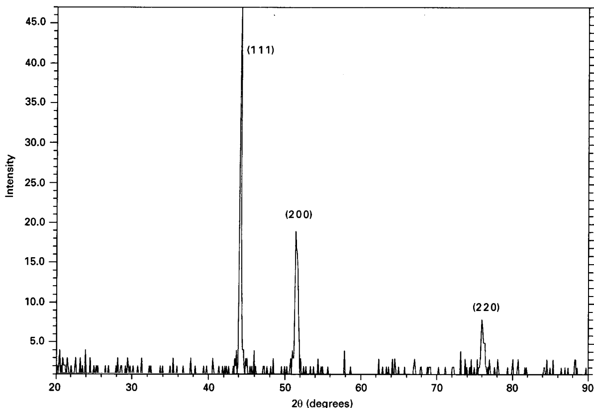
Figure 1 X-ray diffraction pattern of Ni 3 Al obtained in this work.
