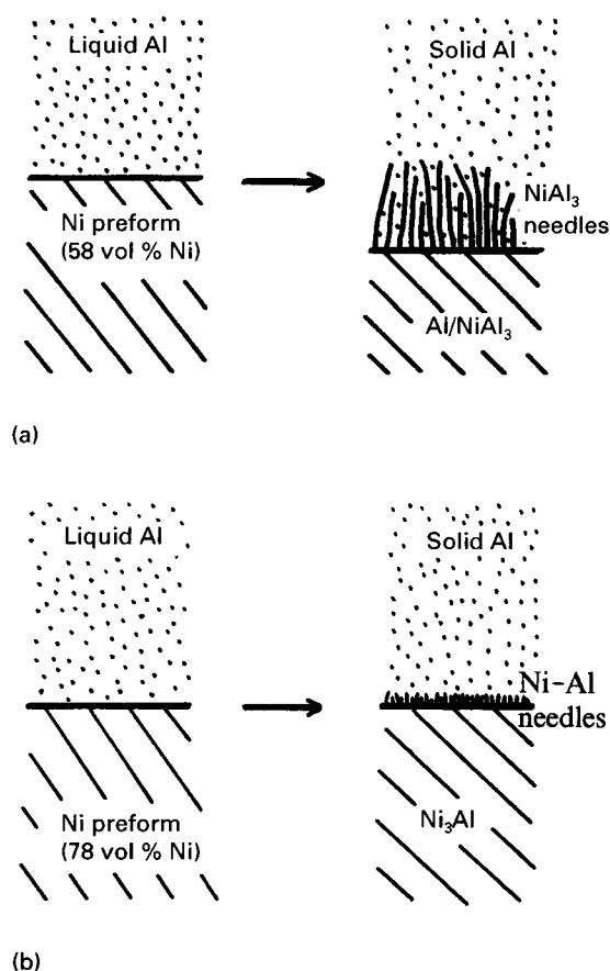
Figure 7 Schematic illustration of the interface between the product and the excess aluminium. (a) The preform contained 58 vol % Ni and the process was not near net-shape. (b) The preform contained 78 vol % Ni and the process was near net-shape.
