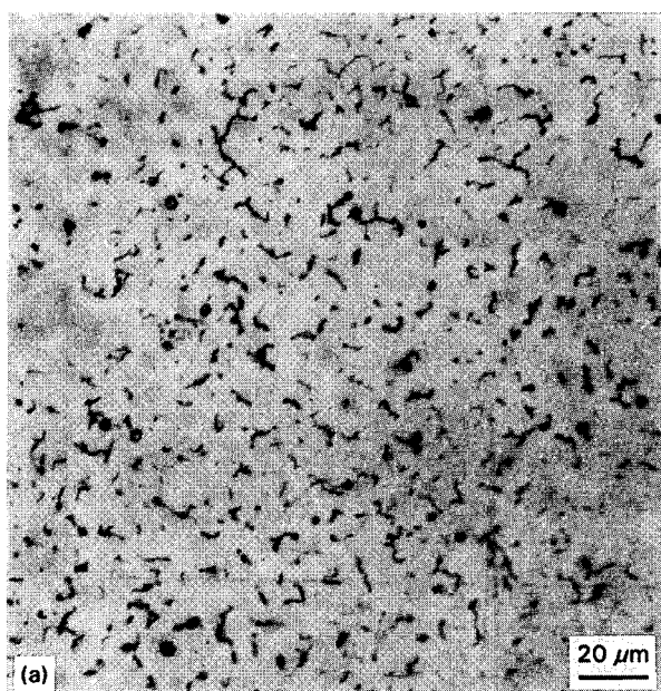
Figure 2 Optical micrographs obtained after light etching of the \text{Ni}_3\text{Al} of this work.
