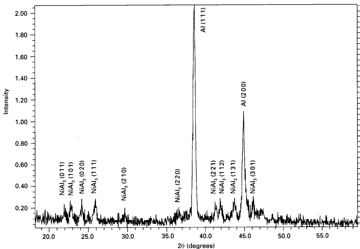
Figure 4 X-ray diffraction pattern of Al/NiAl 3 obtained in this work.
